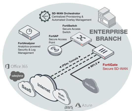
Enterprise Branch Secure SD-WAN Deployment
